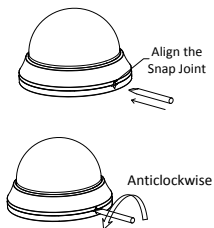
Figure 2-12 Disassemble the Camera
