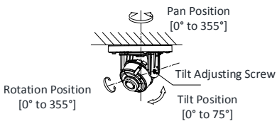
Figure 2-10 3-Axis Adjustment
