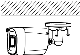
Figure 2-5 Attach the Camera to the Ceiling
