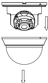
Figure 2-13 Remove the Bubble and the Black Liner
