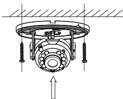
Figure 2-15 Attach the Mounting Base to the Ceiling
