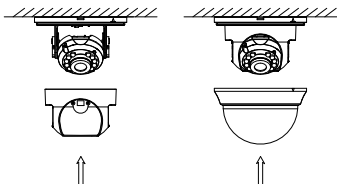
Figure 2-17 Put the Black Liner and the Bubble Back
