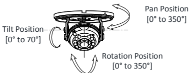
Figure 2-16 3-Axis Adjustment
