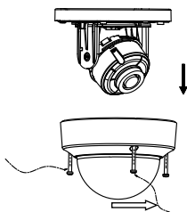
Figure 2-8 Remove the Bubble
