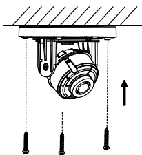
Figure 2-9 Attach the Mounting Base
