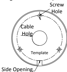
Figure 2-1 Drill Template
