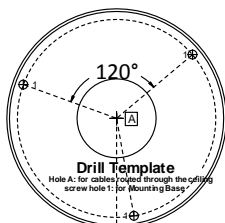
Figure 2-7 Drill Template
