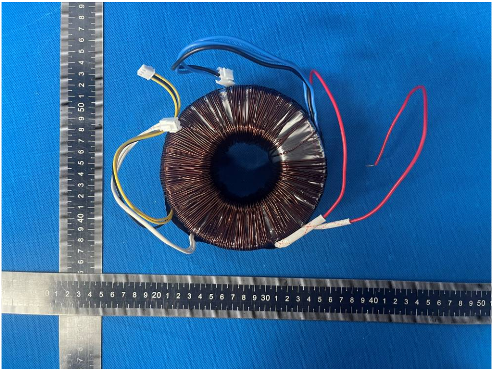
Photo 37. Transformer PG240HK view
