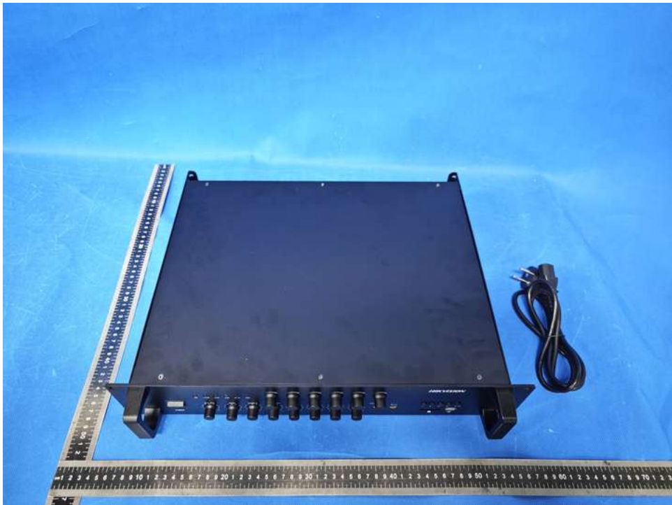
Photo 1. 1.Overall view
