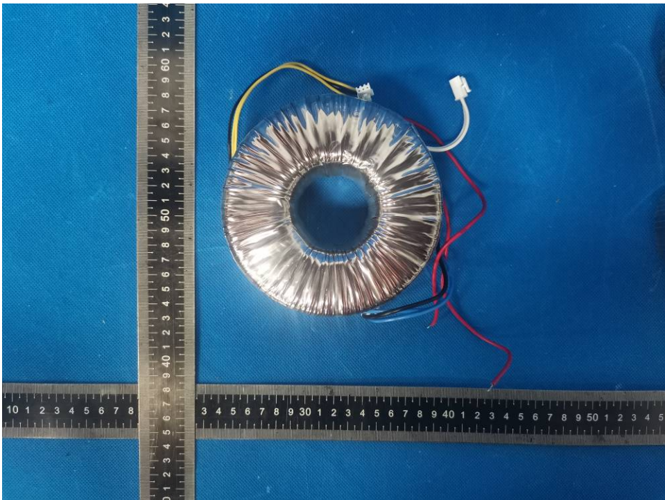
Photo 34. Transformer PG240HK view
