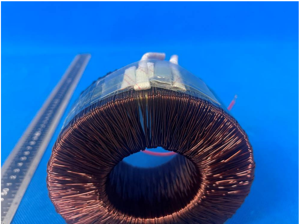
Photo 45. Transformer PG240HK view
