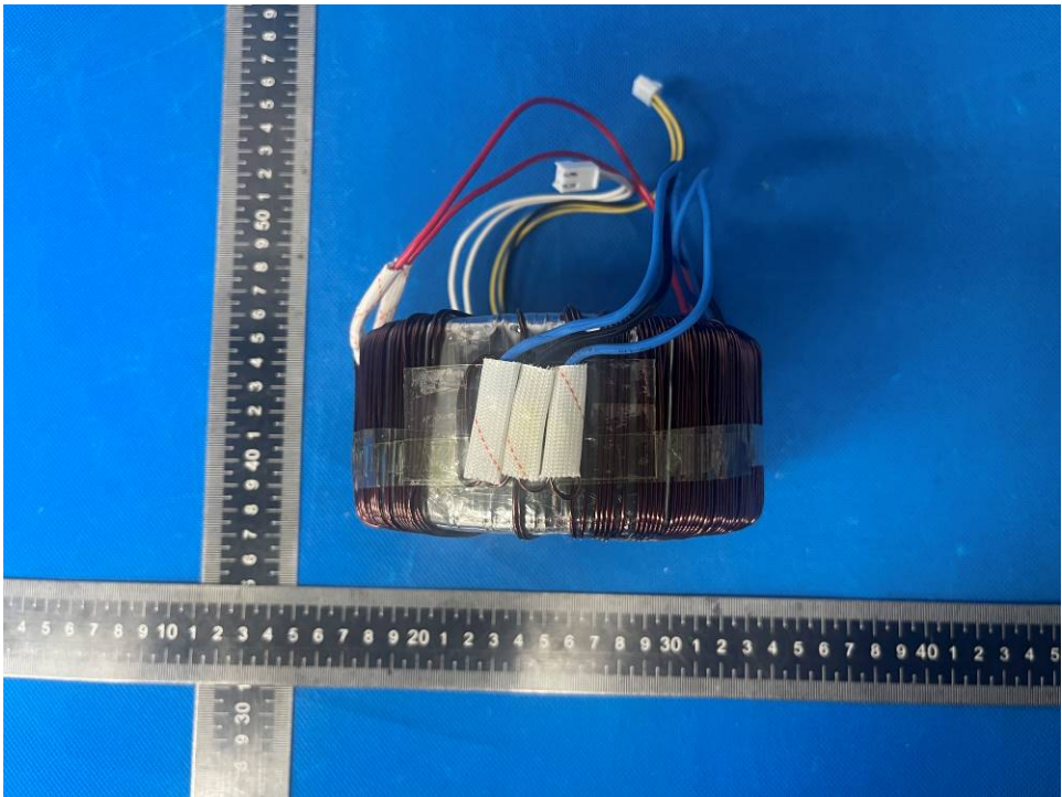
Photo 40. Transformer PG240HK view
