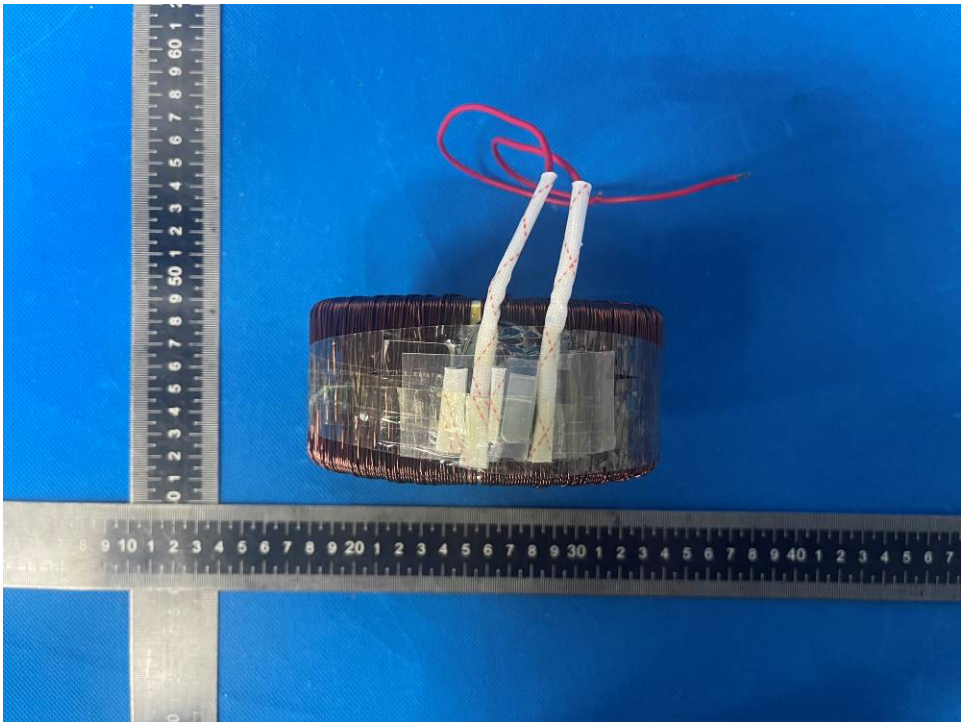
Photo 44. Transformer PG240HK view
