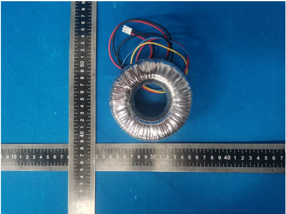
Photo 49. Audio Transformer PG250 view
