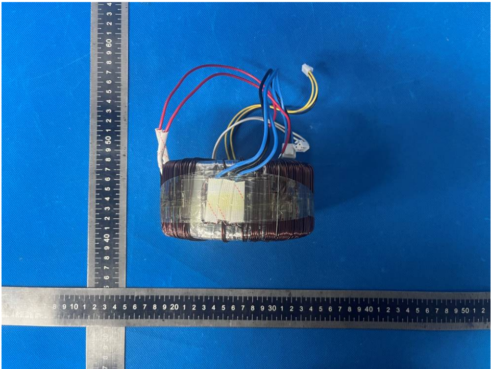
Photo 38. Transformer PG240HK view
