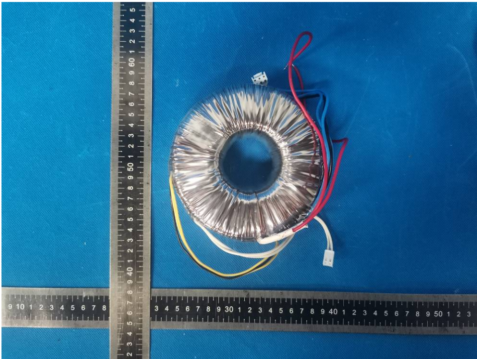
Photo 33. Transformer PG240HK view
