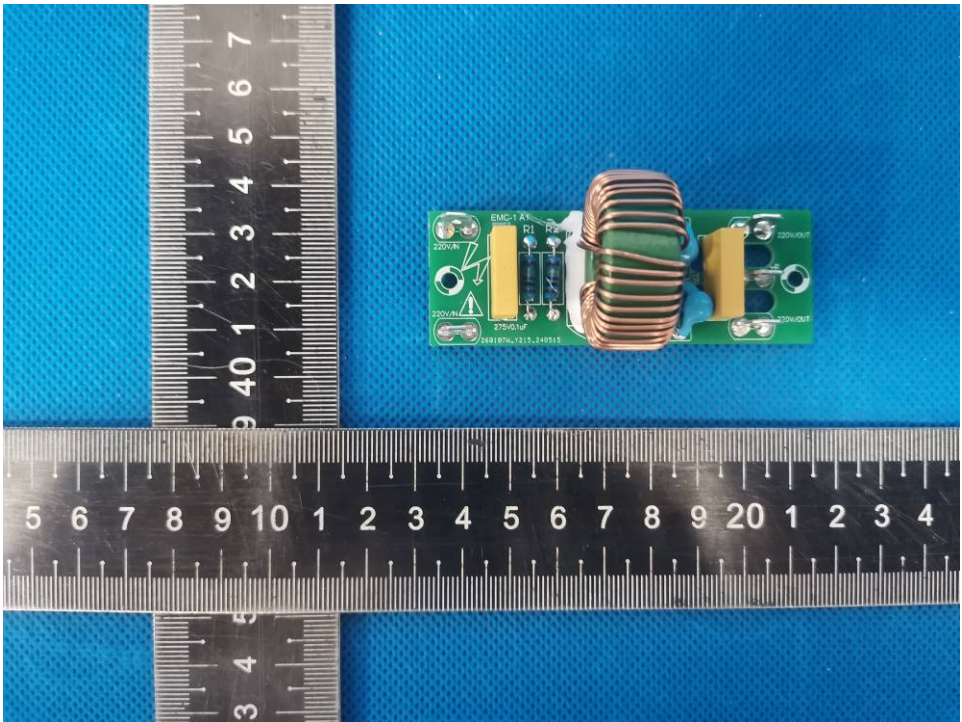
Photo 19. PCB view
