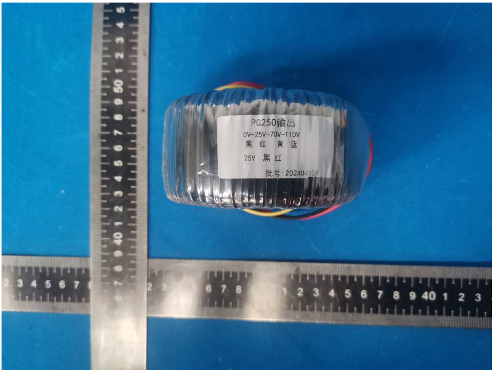
Photo 50. Audio Transformer PG250 view
