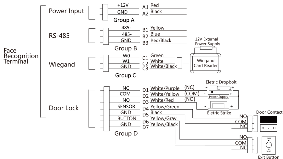
Figure 4-1 Device Wiring
