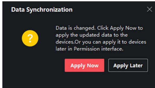
Figure 9-8 Data Synchronization
