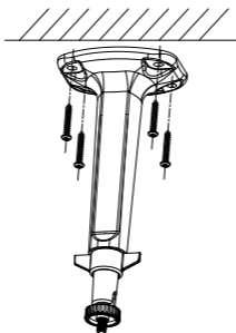
Figure 2. 4 Fix the Bracket on the Ceiling
