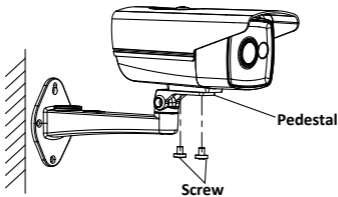
Figure 2. 2 Secure the Camera on the Bracket
