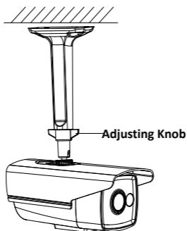
Figure 2. 6 Fix the Camera to the Bracket
