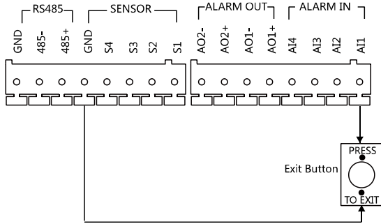
Exit Button Wiring for DS-KD8102-V/DS-KD8002-VM (1)
