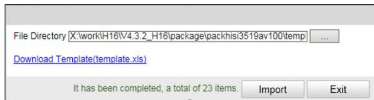
Figure 11-3 Import Completed
