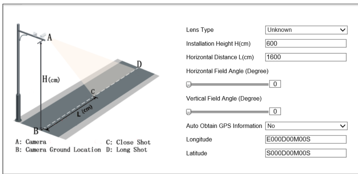
Figure 6-1 Installation Parameters
