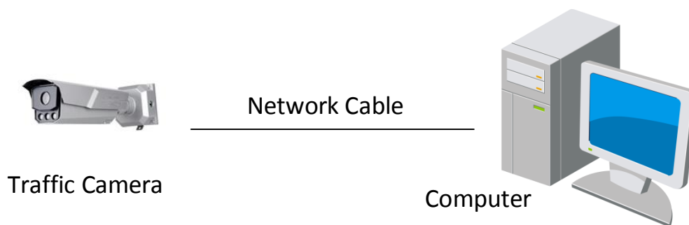
Figure 1-1 Connecting Directly
