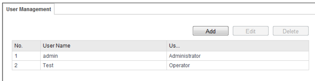
Figure 14-2 User Management
