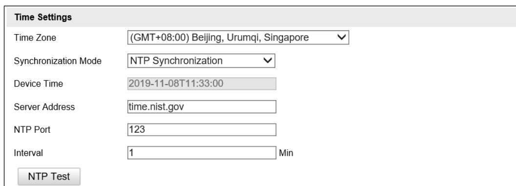
Figure 6-8 NTP Synchronization
