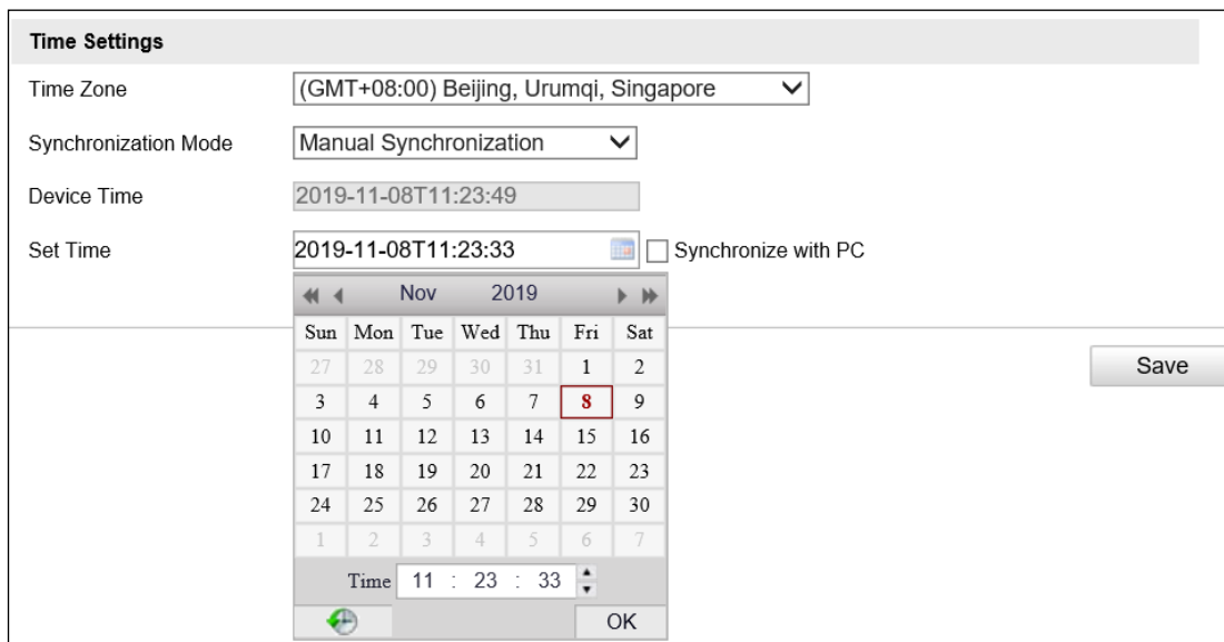
Figure 6-7 Manual Synchronization
