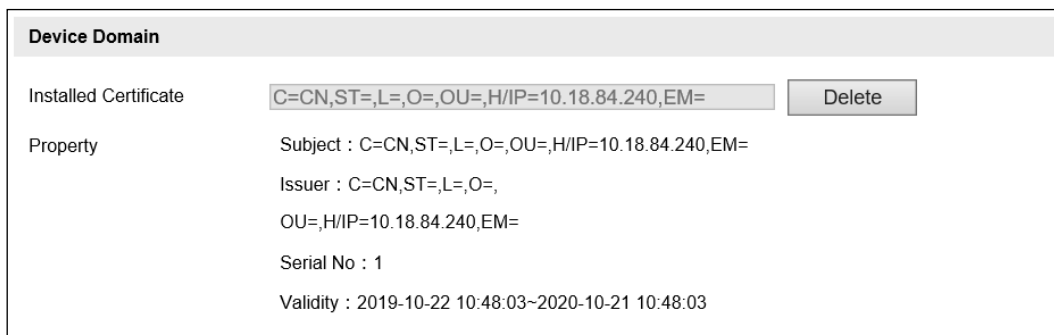
Figure 6-5 HTTPS Configuration
