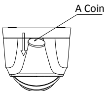
Figure 2-10 Pry the Mounting Base
