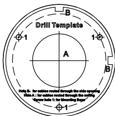
Figure 2-15 The Drill Template
