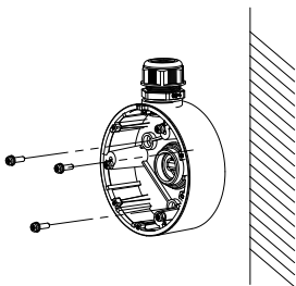
Figure 2-8 Secure the Junction Box
