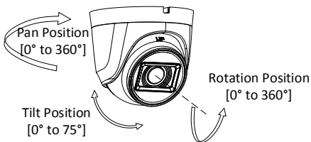
Figure 2-14 3-Axis Adjustment
