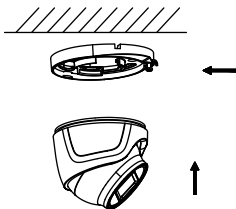
Figure 2-21 Secure the Camera
