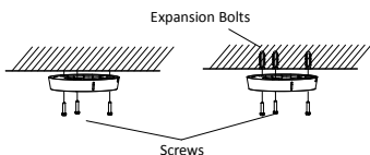
Figure 2-4 Attach the Mounting Base to the Ceiling
