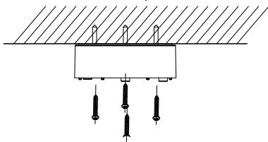
Figure 2-17 Secure the Junction Box's Body
