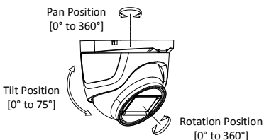
Figure 2-22 3-Axis Adjustment
