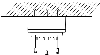
Figure 2-18 Combine the Junction Box
