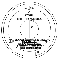
Figure 2-7 The Drill Template
