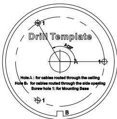
Figure 2-11 Drill Template
