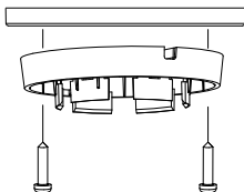
Figure 2-16 Install the Mounting Base
