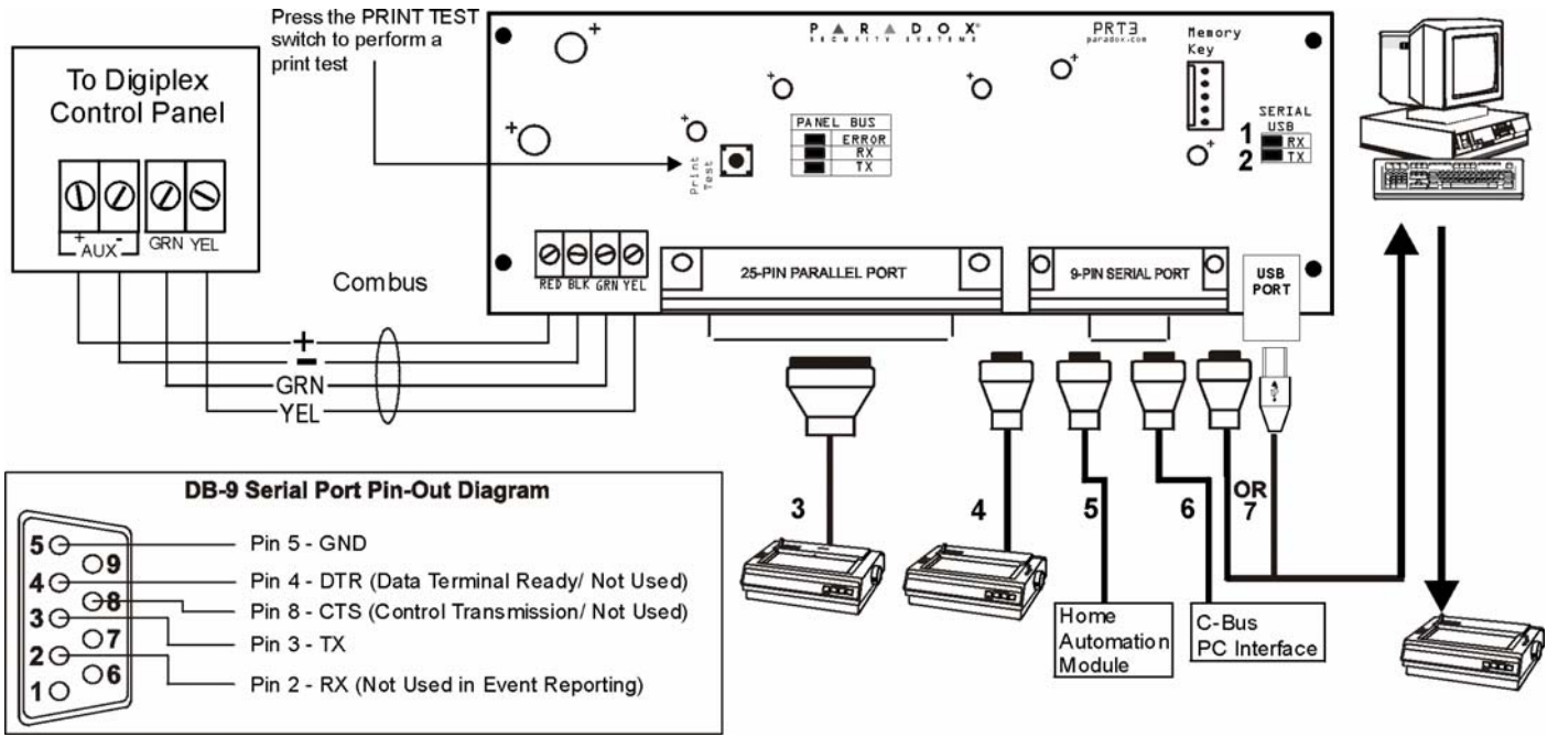
Figure 2: .PRT3 Connection
