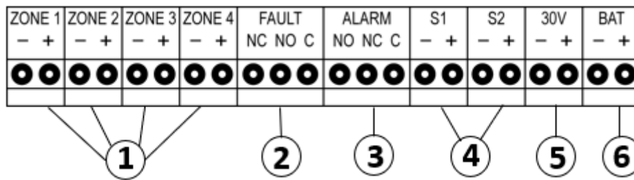
Figure 5: Terminal schema IRON02/04
