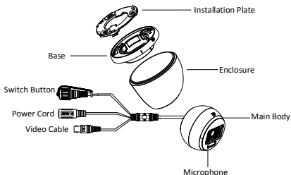
Figure 1-5 Overview of Type V Camera
